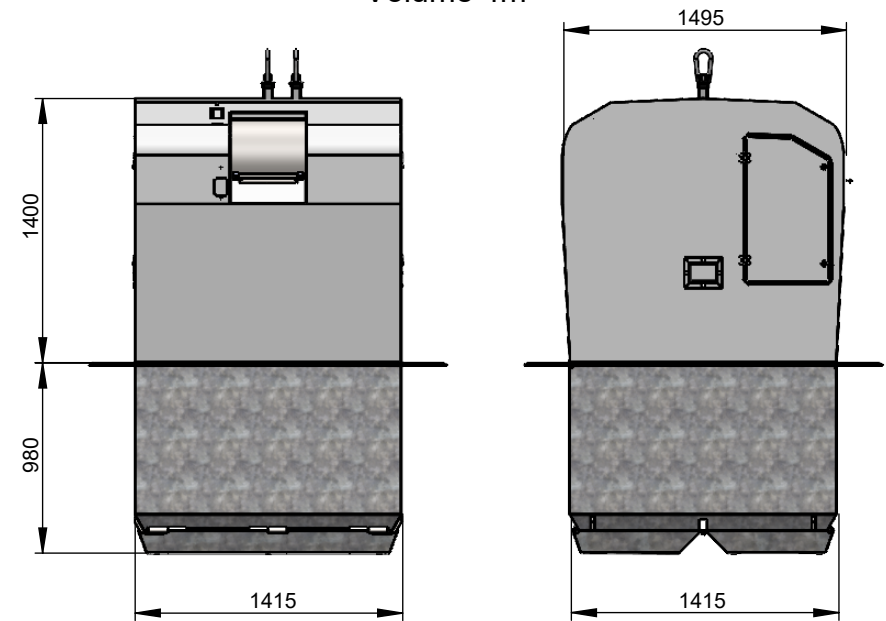
Volume 4m 3
